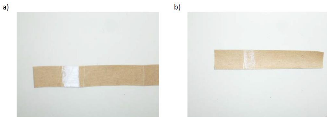
Fig 3. Photographs of specimens of glass-coated abrasive paper specimens exhibiting: a) a dense, chalky white powder deposit; b) a light powder deposit.
